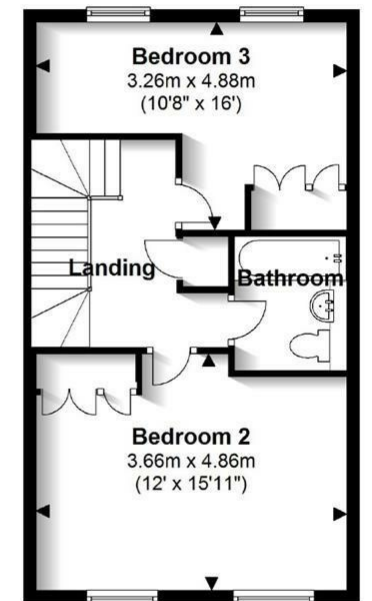
Second Floor Approx. 43.7 sq. metres (470.7 sq. feet)
